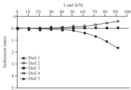
Fig. 8: Load-settlement relation on base layer model non-geogrid
