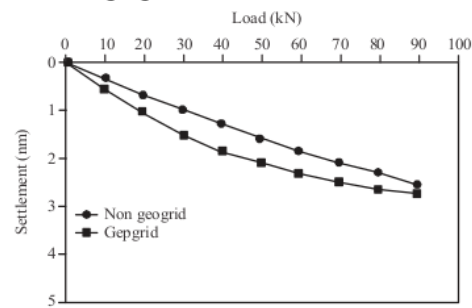
Fig. 11: Load-settlement comparison of geogrid-reinforced base and non-geogrid
