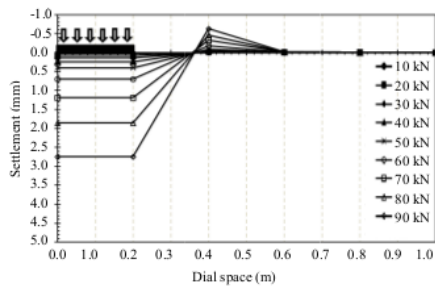
Fig. 9: Deformation behavior per load phase of stabilized laterite soil non-geogrid
