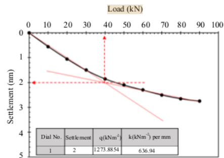
Fig. 10: Modulus value of stabilized laterite soil non-geogrid
