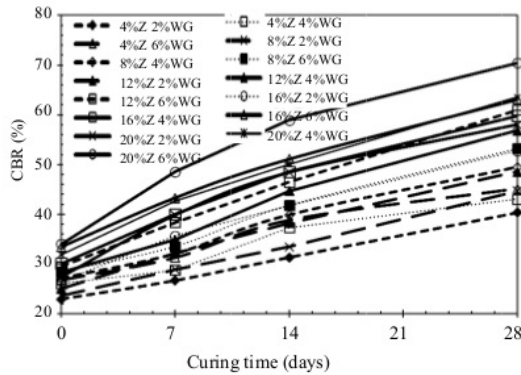
Fig. 3: CBR test result
