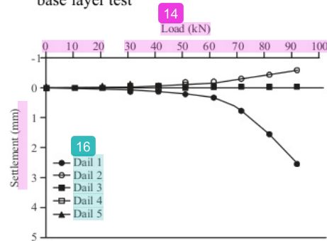
Fig. 5: Load-settlement relation on base layer model with geogrid reinforcement
